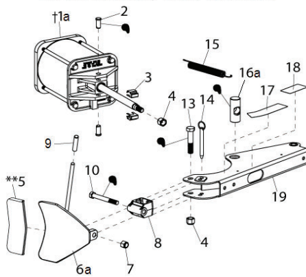
BL Arm Assembly (Foot Operated)
