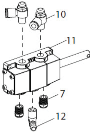
Clamp Control Pedal Valve Assembly
