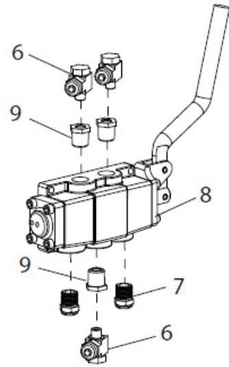
Bead Loosener Arm Valve Assembly
