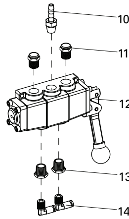
Robo Arm Valve Assembly
