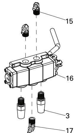
Bead Loosener Arm Valve Assembly
