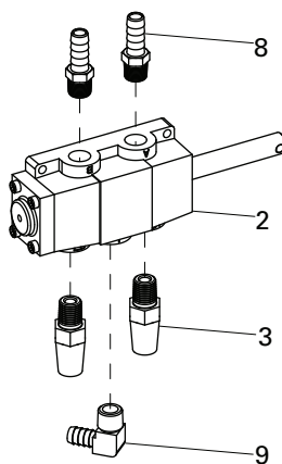
Air Motor Pedal Valve Assembly
